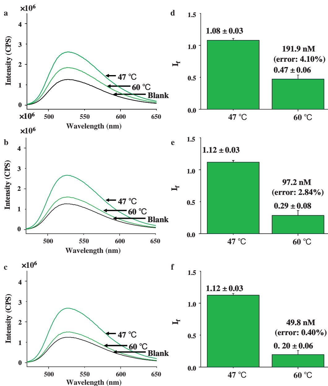
Fig. 5. (a–c) Fluorescence spectra of the supernatants obtained by using the RFMP- \text{Fe}_3\text{O}_4/\text{Al}_2\text{O}_3 MNPs as the detection probes to interact with the released DNA from the samples A, B, and C. Panels (d–f) are their corresponding bar graphs. Three duplicates were conducted for each experiment.
